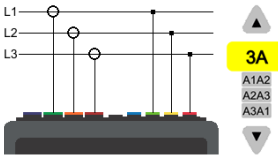
Three-phase 3 wires (L1, L2, and L3)
