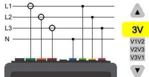
Three-phase 4 wires (L1, L2, L3, and N)
