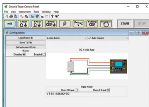
4-POINT-RESISTANCE
